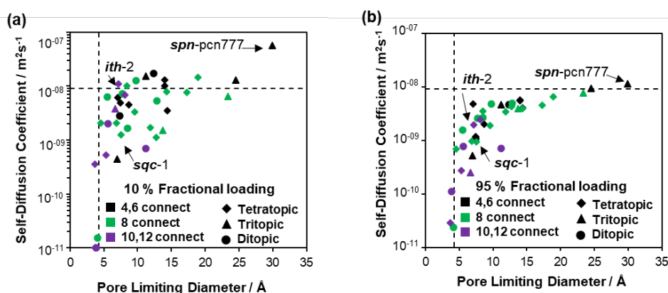
Figure 1: Self-diffusion coefficients of propane versus pore limiting diameter for 38 Zr_6 MOFs at (a) 10% and (b) 95% fractional loading.
