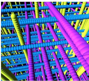
Figure 1: (Right) One of the random networks where passive tracers diffuse anomalously. (Left) Pictorial representation of our model for the exciton diffusion in perovskite layers.
