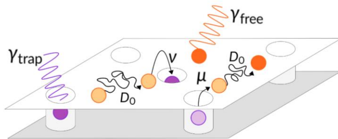
Figure 1: (Right) One of the random networks where passive tracers diffuse anomalously. (Left) Pictorial representation of our model for the exciton diffusion in perovskite layers.
