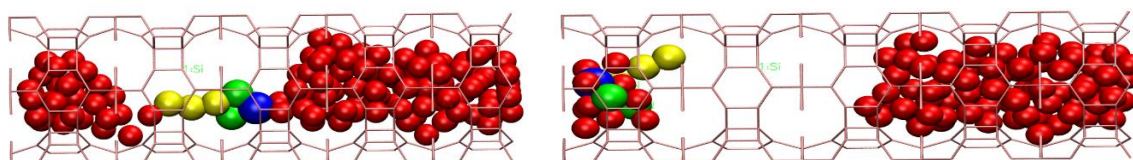
Figure 2: Molecular diffusion before water extrusion from 18MR channel. A time step for snapshots is 40 ps.
