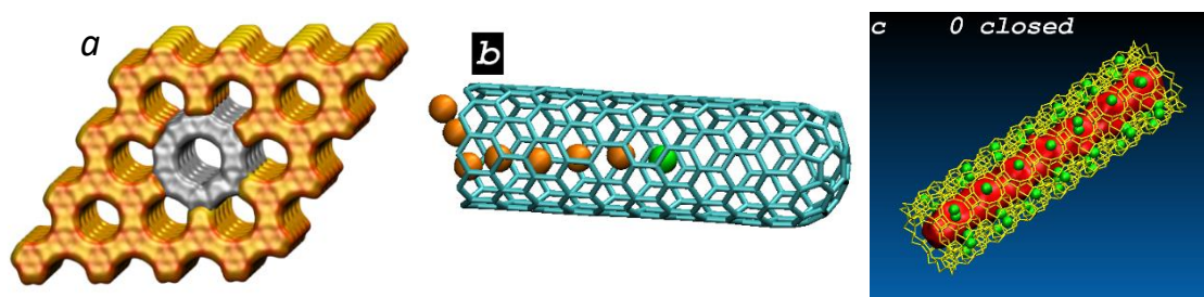
Figure 1: Nano-objects under consideration: (a) nanoparticle, (b) captured CNT, (c) nanotube. Coloured balls show water molecules.
