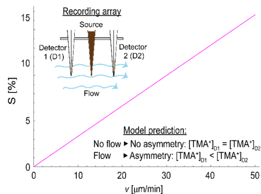
Figure 1. FloD method: recording setup and model prediction. We used the D typical for the tetramethylammonium (TMA) probe molecule. We expect to be able to reliably detect flow values of about 10 \mu\text{m}/\text{min} in the ECS. Such flow or higher would play a significant role in the clearance of harmful macromolecular metabolites. D1 and D2 are the detectors of tetramethylammonium.
