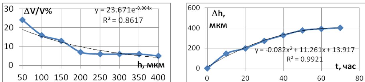
Fig. 1. a ) the dependence of the absorption level of AW in the surface layers of steel (38XM10A) depth of nitriding layer ( t^0 process 560^0\text{C} ); b ) the dependence of the thickness of the layer with altered properties from the time of nitriding (at t^0 = 500^0\text{C} ) obtained by the change of speed v_R of surface acoustic waves in steel (40XHMA).
