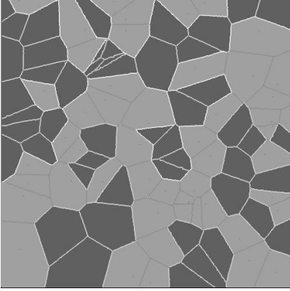
Figure 9: Polycrystalline composite material created by Voronoi construction in two dimensions. Dark grey areas represent the ionic conductor grains and light grey areas represent the insulator grains.
