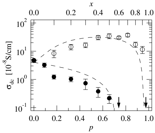
Figure 6: Results of the continuum percolation approach (dashed lines) compared to the experimental results for the dc conductivity at 433 K, after [11]. The arrows indicate the compositions where the dc conductivities fall below the detection limit.
