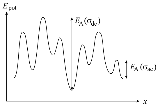
Figure 12: Potential landscape for the movement of the Li ions. The ac conductivity probes dynamics on shorter length scales and thus gives lower activation energies than the dc conductivity.
