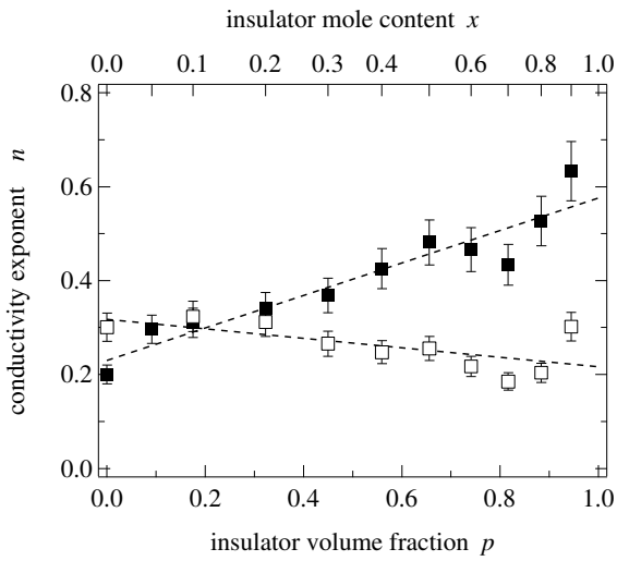
Figure 4: Exponent n (cf Eq. (1)) for the ac conductivity of microcrystalline (■) and nanocrystalline (□) (1-x)\text{Li}_2\text{O}:x\text{B}_2\text{O}_3 composites vs insulator volume fraction.
