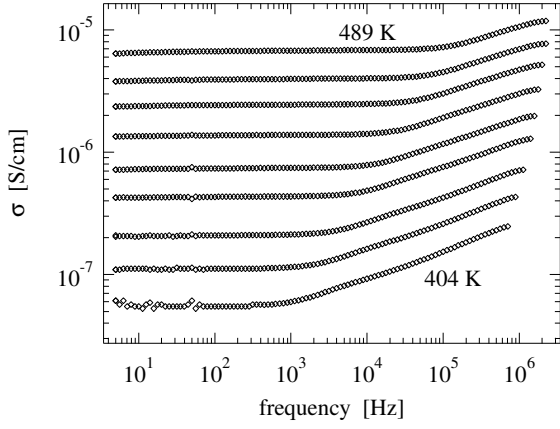
Figure 1: Real part of the conductivity vs frequency for nanocrystalline (1-x)\text{Li}_2\text{O}:x\text{B}_2\text{O}_3 for x = 0.6 . The corresponding temperatures are 489 K, 478 K, 468 K, 457 K, 446 K, 436 K, 425 K, 414 K and 404 K (top to bottom).
