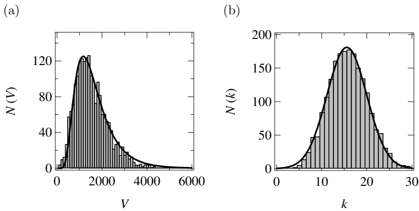
Figure 10: The distribution of (a) grain volumes and (b) coordination numbers found for a Voronoi system on a lattice of 150^3 lattice sites with 2000 Voronoi cells. The volumes are given in units of the volume of an elementary lattice cell. The solid lines represent fits with a log-normal distribution of grain volumes (Eq. (4)) and a normal distribution of coordination numbers (Eq. (5)), respectively.
