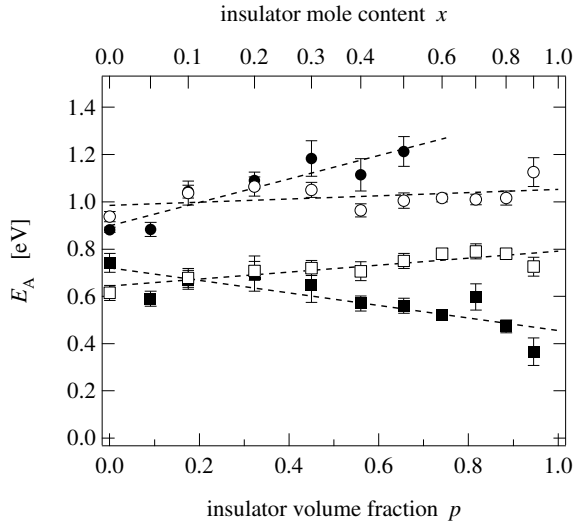
Figure 3: Activation energies of the dc (circles) and ac (squares) conductivity of microcrystalline (full symbols) and nanocrystalline (open symbols) (1-x)\text{Li}_2\text{O}:x\text{B}_2\text{O}_3 composites vs insulator volume fraction.
