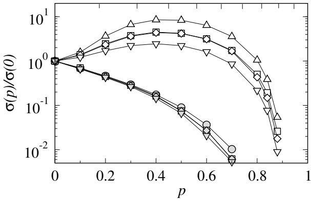
Figure 8: Numerical results of the normalized dc conductivity \sigma(p)/\sigma(0) vs insulator volume fraction p in the brick-layer type percolation model for different grain sizes a and enhancement factors \tau = \sigma_A/\sigma_B . In all cases the interface thickness \lambda = 1 nm is fixed. Nanocrystalline grains: \triangle a = 10 nm, \tau = 200 ; \square a = 10 nm, \tau = 100 ; \diamond a = 20 nm, \tau = 200 ; \nabla a = 20 nm, \tau = 100 ; Microcrystalline grains: \bullet a = 10 \mu\text{m} , \tau = 200 ; \blacksquare a = 10 \mu\text{m} , \tau = 100 ; \blacklozenge a = 20 \mu\text{m} , \tau = 200 ; \blacktriangledown a = 20 \mu\text{m} , \tau = 100 [20].
