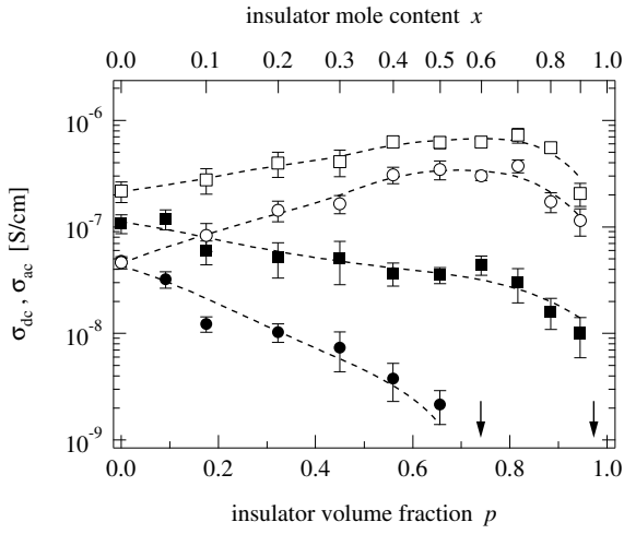
Figure 2: Dc (circles) and ac (squares) conductivities of microcrystalline (full symbols) and nanocrystalline (open symbols) (1-x)\text{Li}_2\text{O}:x\text{B}_2\text{O}_3 composites vs insulator volume fraction at 433 K. Dashed lines are drawn to guide the eye. The arrows indicate the compositions where the dc conductivity of the micro- and nanocrystalline materials show a sharp drop and fall below the detection limit.
