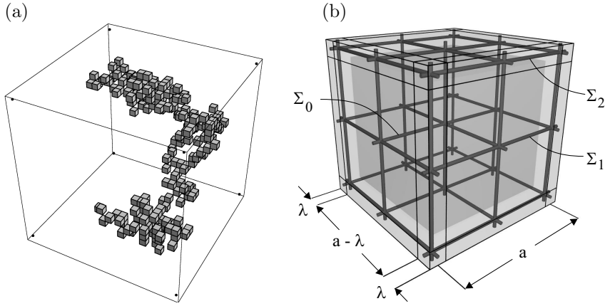
Figure 7: (a) The largest cluster of insulating particles for the brick-layer type model in three dimensions at the critical concentration. (b) A single grain and the bonds assigned to conduction in the interior of the grains, along the sides and along the edges of the grain [20].
